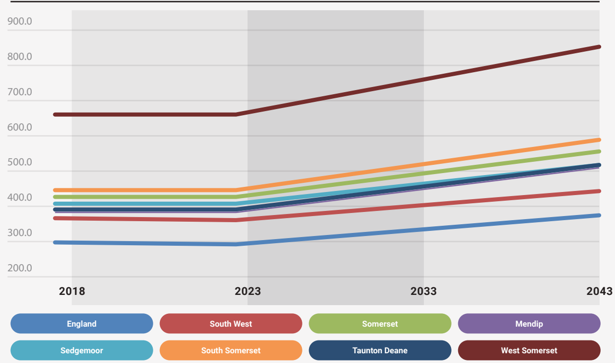
Figure 17 - OADR Predictions
